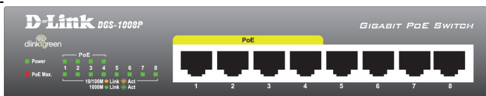
Figure 1 – DGS-1008P Front Panel
